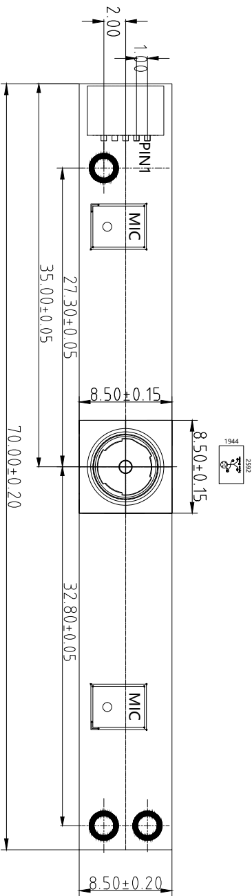
TOP VIEW
